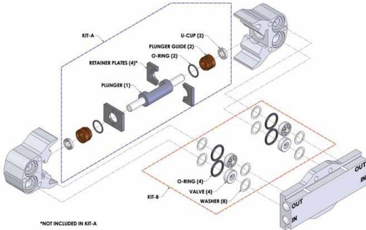
Repair Parts Illustration for Plunger Pump
