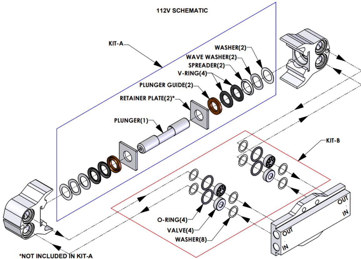
Repair Parts Illustration for Plunger Pump Note: 217V internal components are the same as 112V internal components
